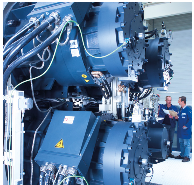
Highly dynamic torque motors on the crown allow for a high level of flexibility.
