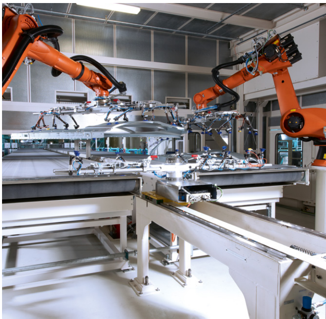
Transfer of finished workpieces from the shuttle to the robot.
