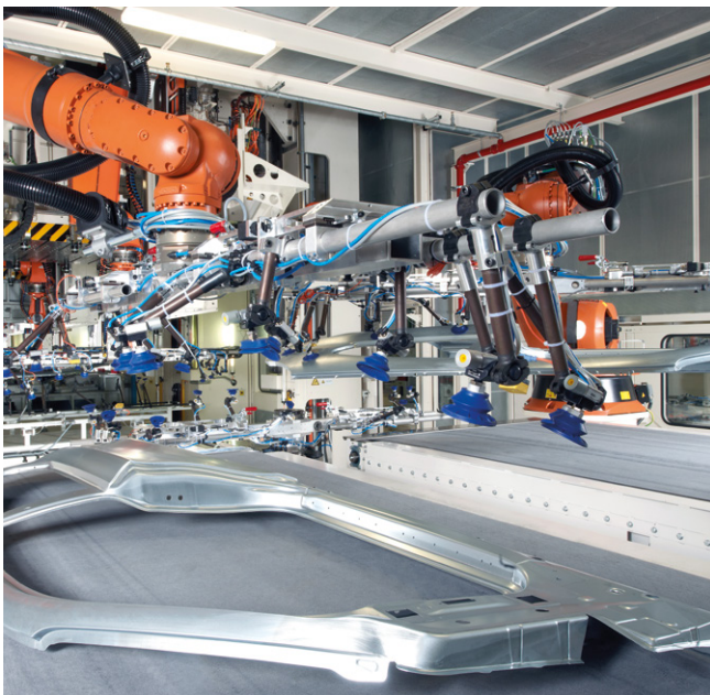
Finished part deposit. The finished workpieces are deposited to the left and right of the conveyor belts by two robots.
